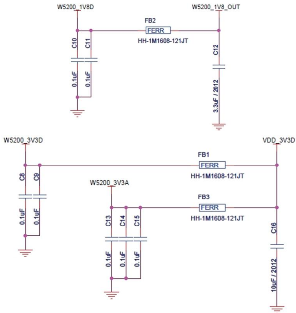
Figure 3 Power Design
