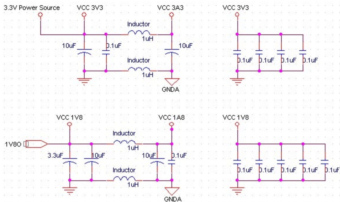
Figure 1.9 Power Design
