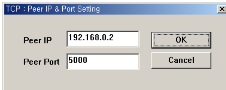
<Fig 3.15> iinChip™ EVB B/D's IP and Listen Port Setting for TCP Loopback Test
