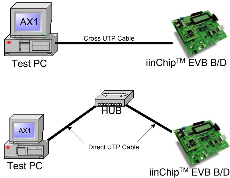
<Fig 3.1> System composition example in LAN interface
