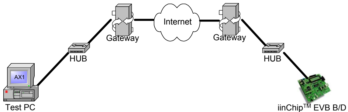
<Fig 3.2> System composition example in WAN interface
