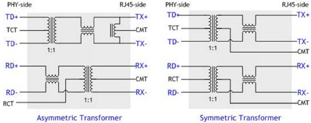
Figure 24 Transformer Type
