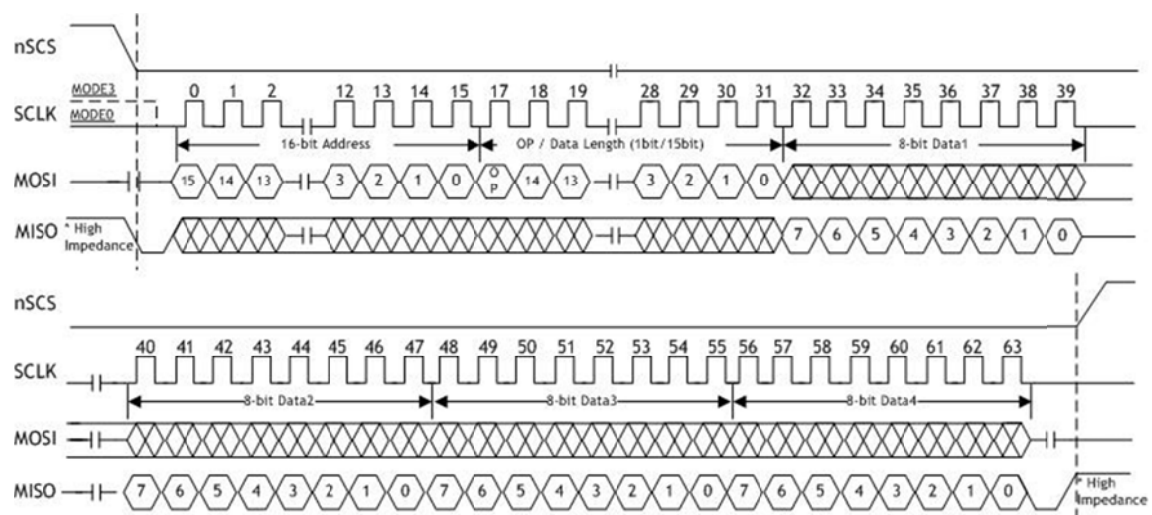
Figure 21 Write Sequence
