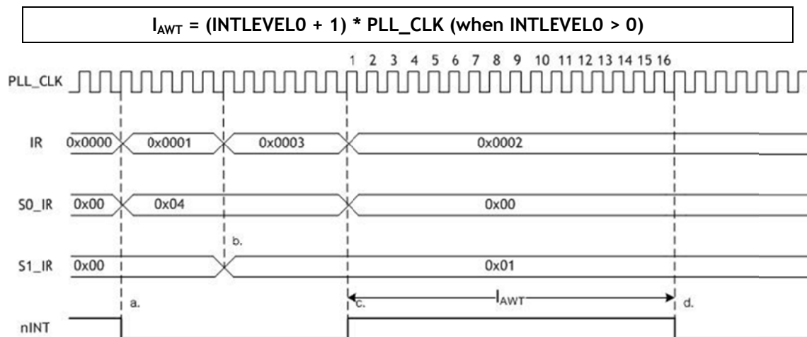
Figure 4 INTLEVEL Timing
