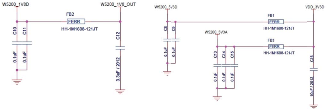
Figure 2 Power Design
