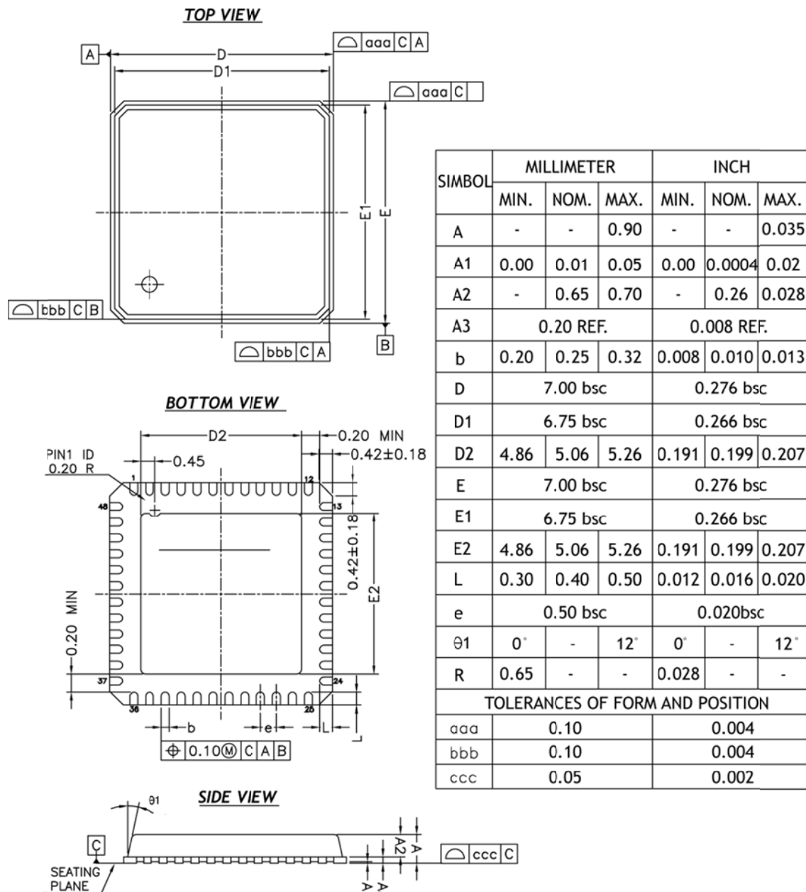
Figure 26 Package Dimensions
