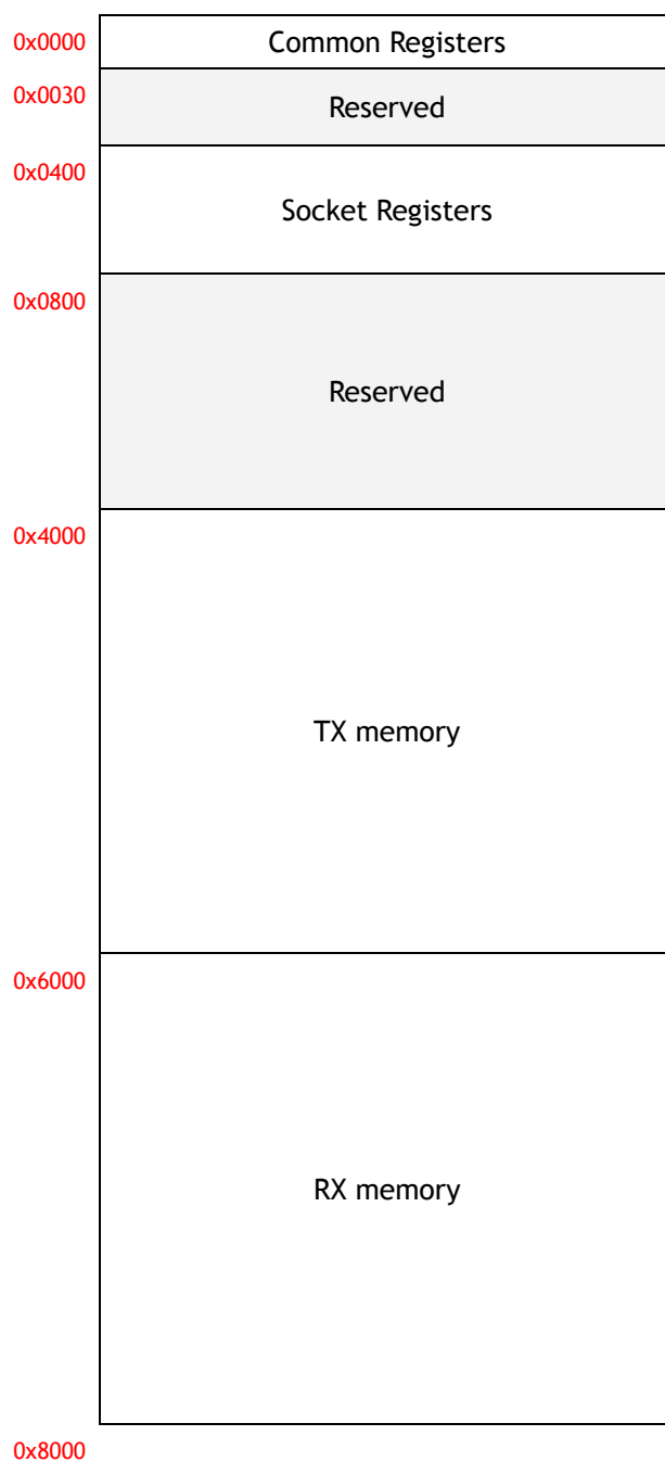
Figure 2. Memory Map
