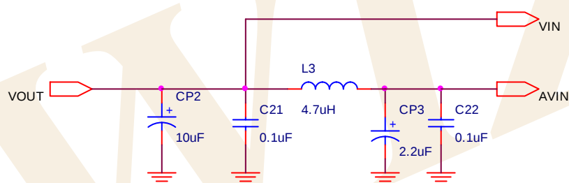
Figure 1-1. Reference Schematic for Power input
