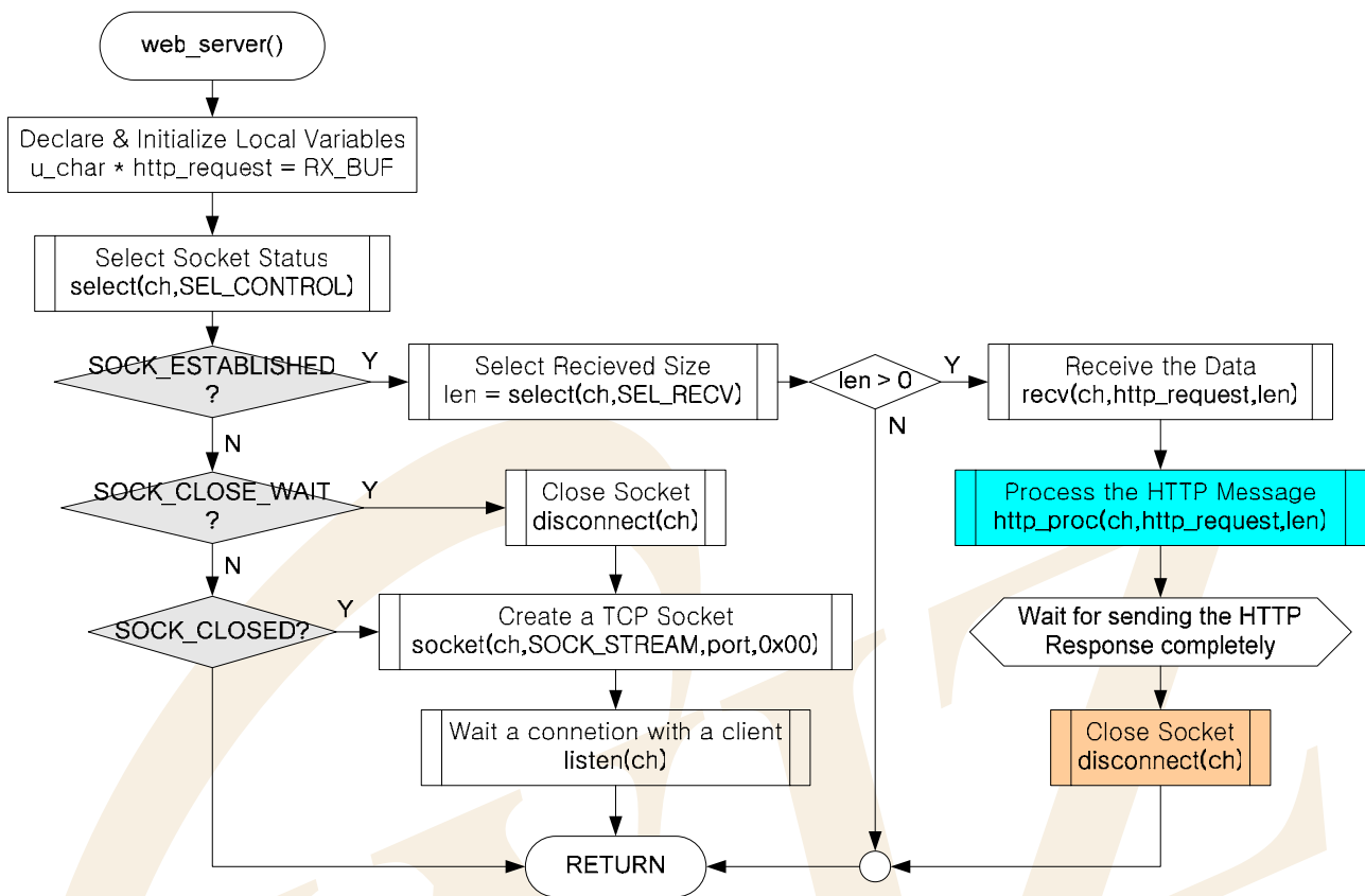
<Fig 3.18: web_server()>
