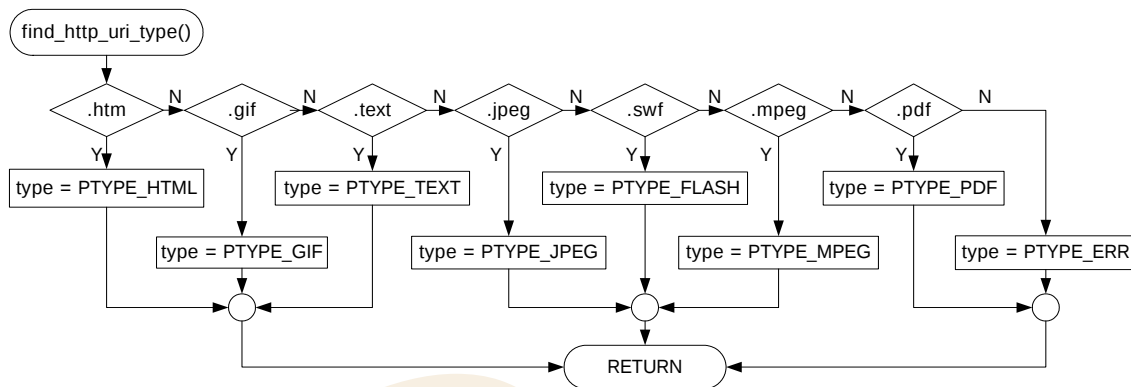
<Fig 3.21: find_http_uri_type()>
