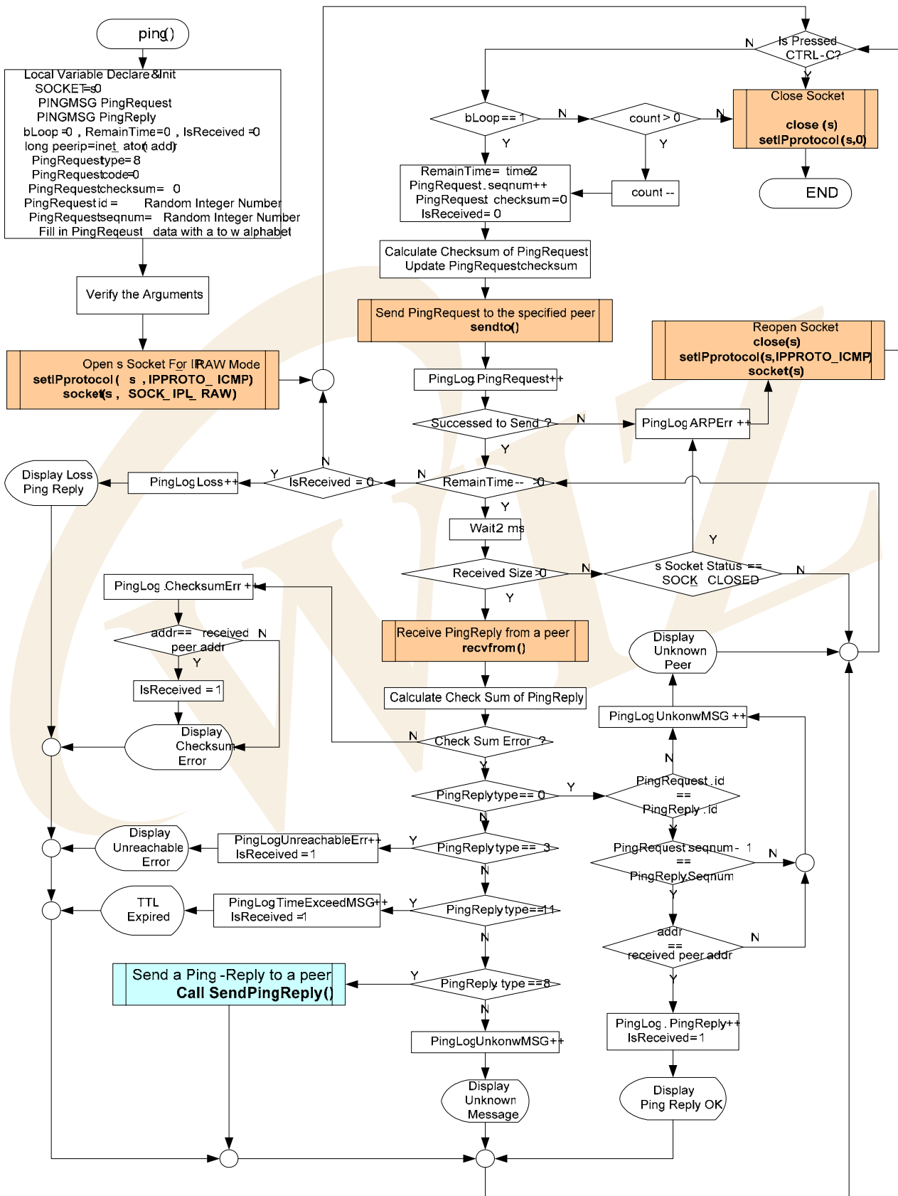
<Fig 3.11: ping(>
