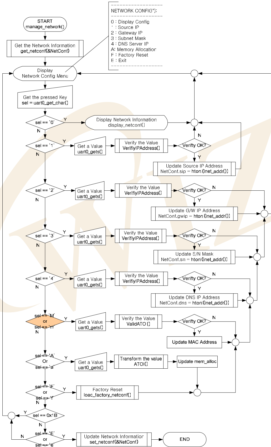
<Fig 3.6: manage_network()>
