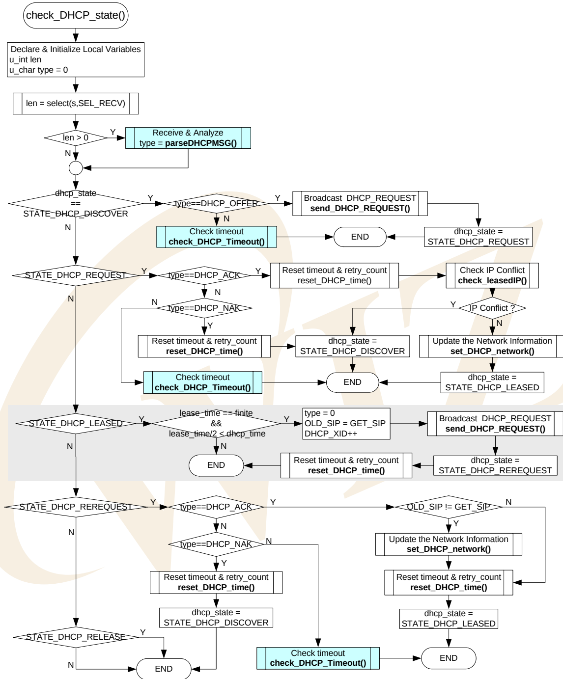
<Fig 3.31: check_DHCP_state()>
