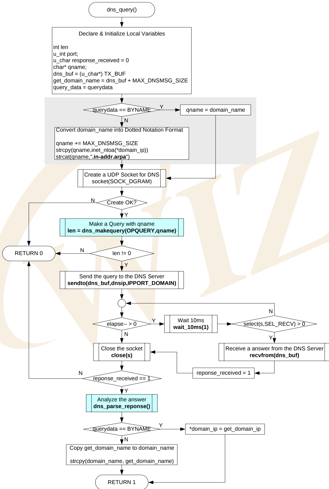
<Fig 3.39: dns_query()>
