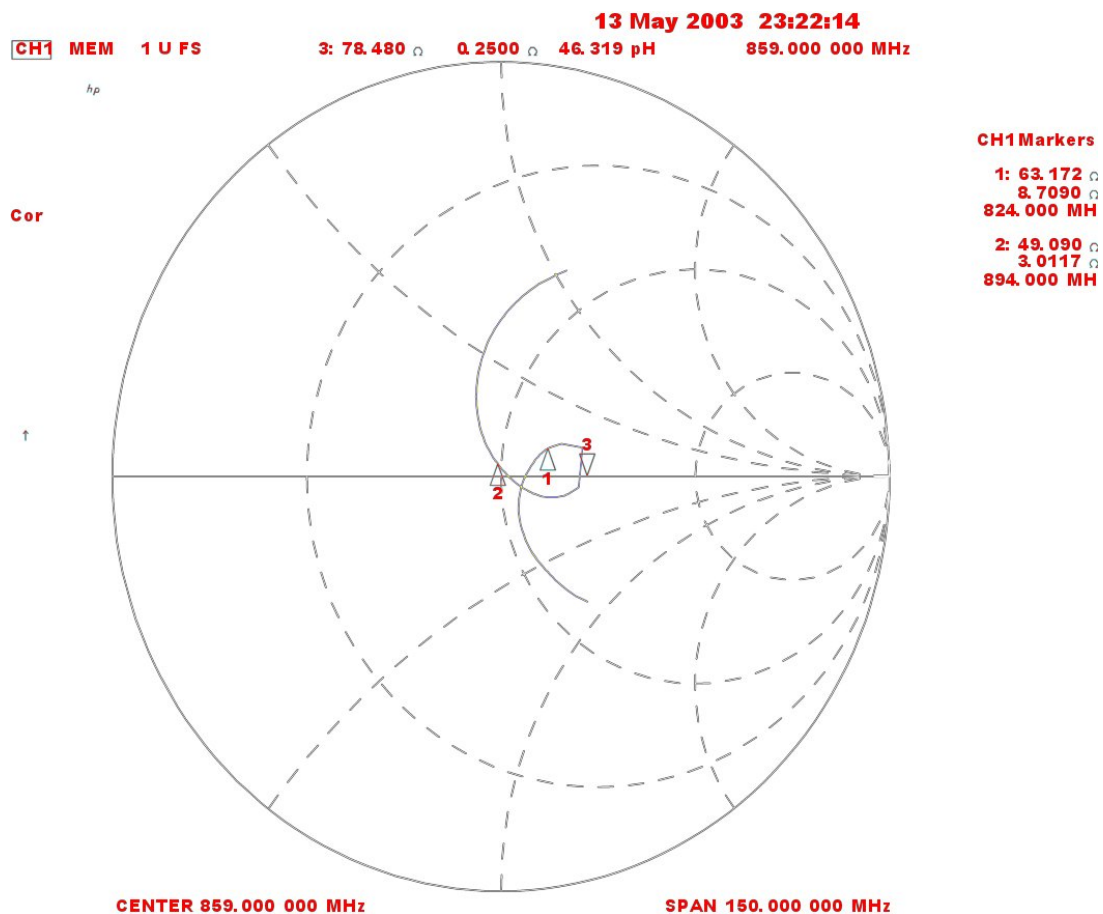
Fig. 2. Smith Chart
