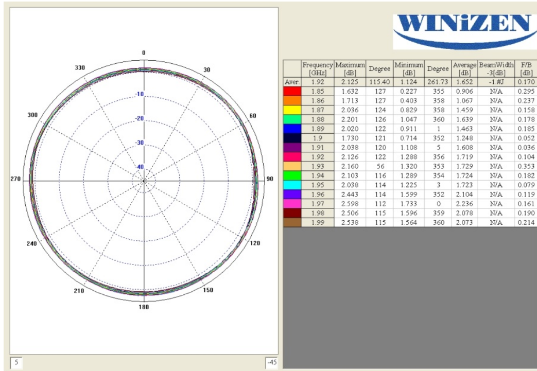
Fig 6. Gain Patterns
