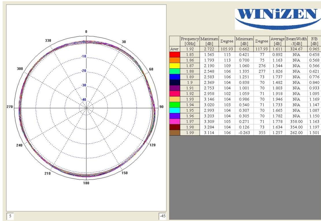
Fig 6. Gain Patterns
