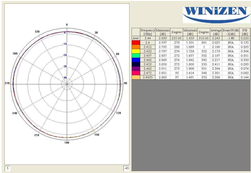
Fig 6. Gain Patterns
