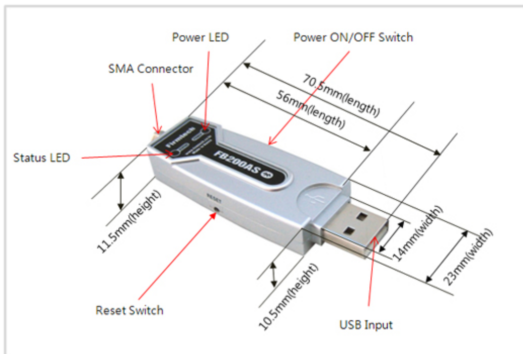
<Figure 4-1 Details and Dimension of FB200AS>
