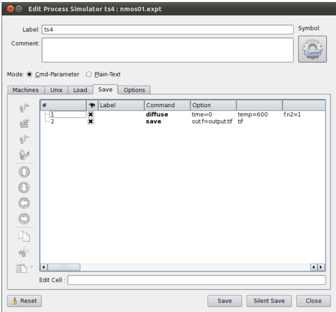
Figure 3.23 Save section of the simulator dialog
