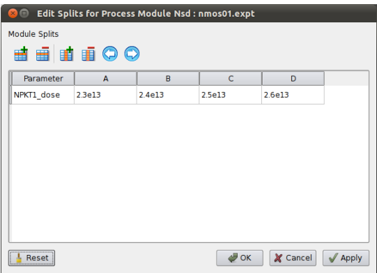
Figure 2.17 Editing splits of a process module
