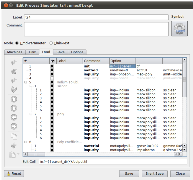
Figure 3.22 Load section in the simulator dialog
