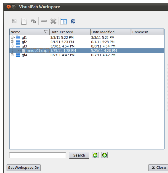
Figure 3.12 Workspace Manager
