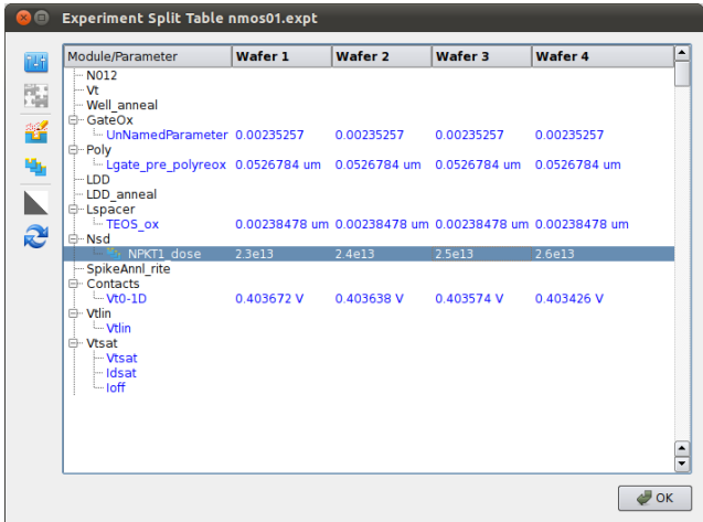
Figure 2.11 Run table of after simulation completes.
