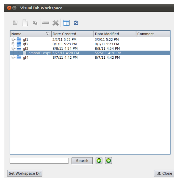
Figure 2.2 Workspace Manager
